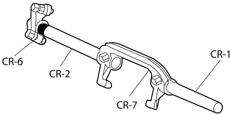
Pedal Adjusting Arm Right Side -310473X
