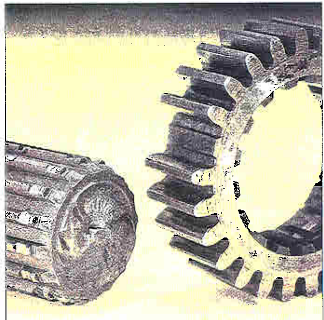
Figure 6—A broken shaft and missing gear teeth indicate shockload.
