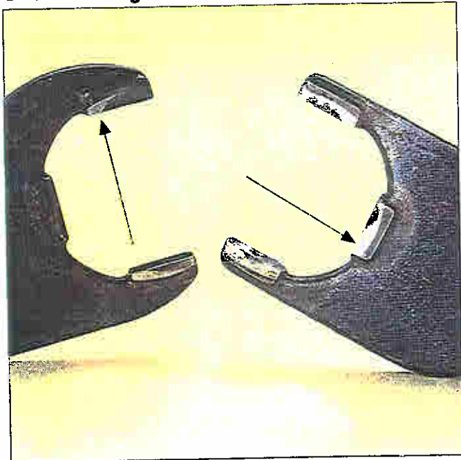
Fork pad wear is caused by over-shifting and clash shifting.
