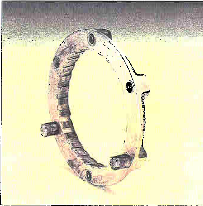
Figure 17—Sheared synchronizer pins are a sign of vibration.
