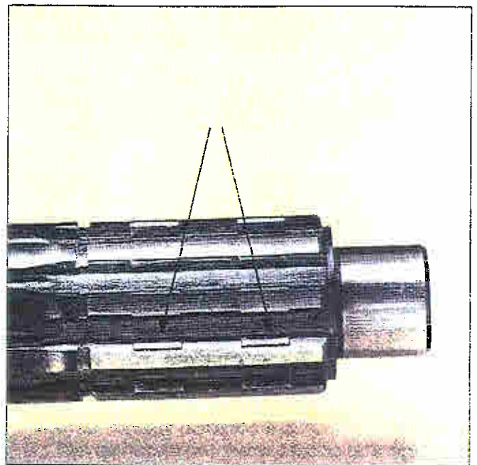
Figure 19—Worn shaft gearlocks can lead to gear jumping.
