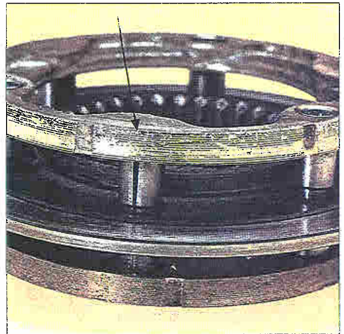
Figure 16—Metal chips are caused by clash shifting or lack of lubrication.
