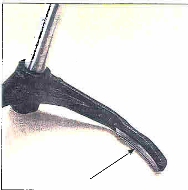
Figure 14—Fork shoe wear.
