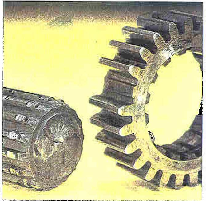
A broken shaft and missing gear teeth indicate shockload.
