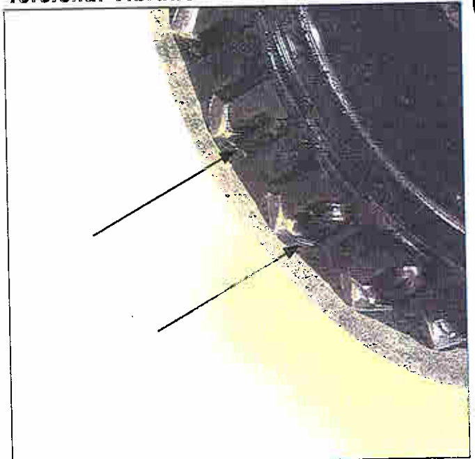
Torsional vibration caused these worn teeth.
